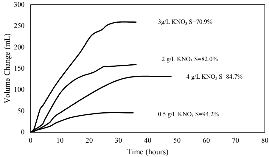
Figure 5-3. Gas generation of permeability tests
